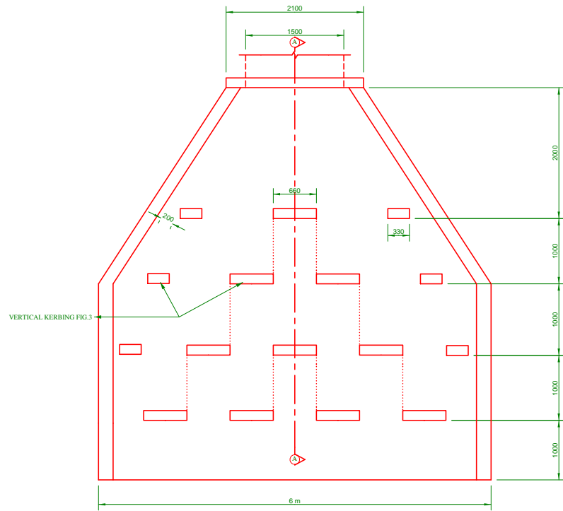
PLAN Scale 1:35
